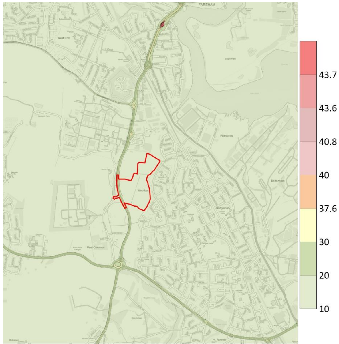
Figure 6-2. Total Long Term Annual Average Nitrogen Dioxide (NO 2 ) Concentration Across the Study Area (µg/m 3 )
